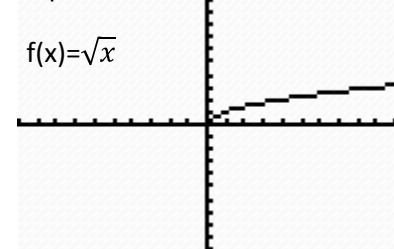
Square-Root Function
