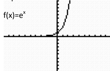
Exponential Function
