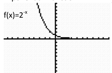
Exponential Function
