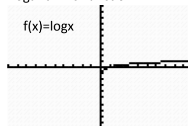
Logarithmic Function
