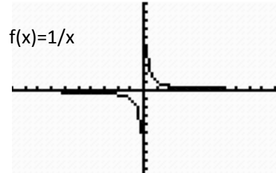
Rational Function
