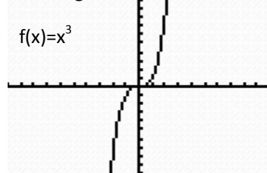
Cubing Function
