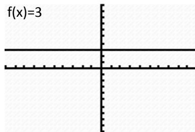
Constant Function
